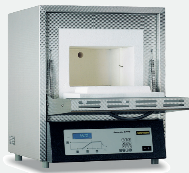
Burnout furnace L 3 from 1989
