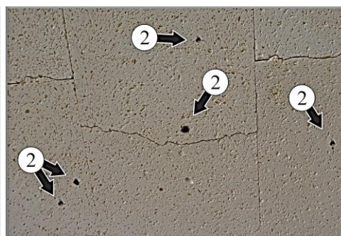
Lunker
